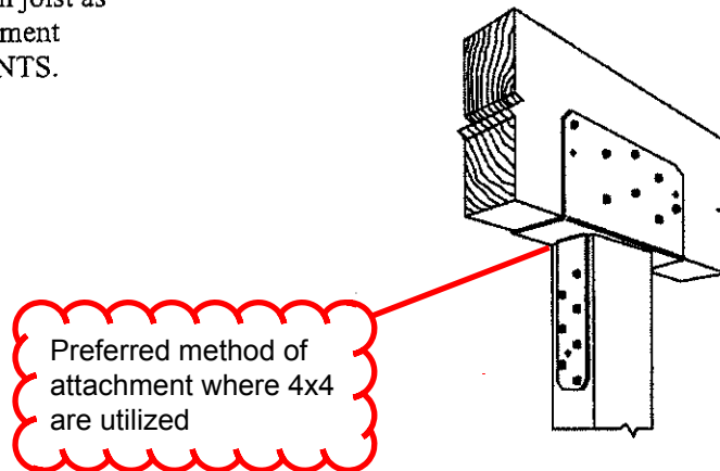
Figure 10: Alternate Approved Post-to-Beam Column Cap Attachment
