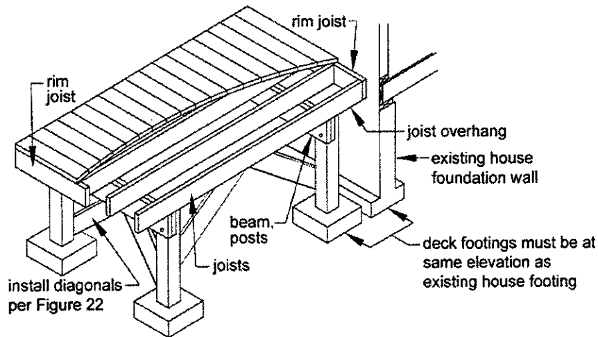
Figure 21: Free-Standing Deck
