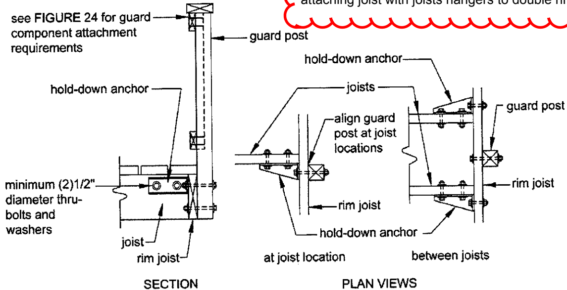
Figure 26: Guard Post to Rim Joist Detail
