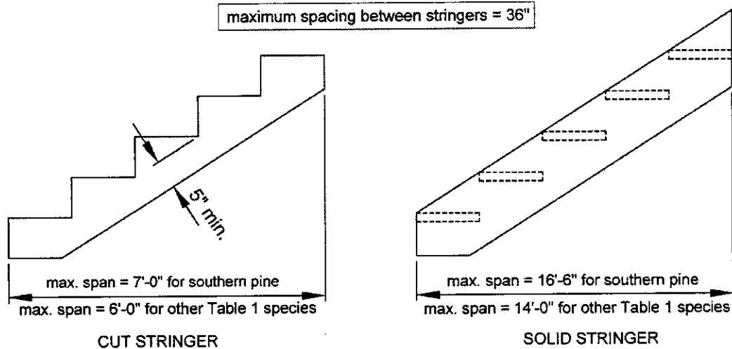
Figure 28: Stair Stringer Requirements
