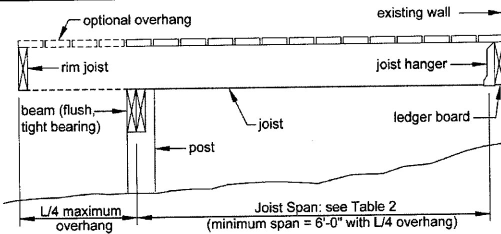
Figure 1A: Joist Span – Deck Attached at House
