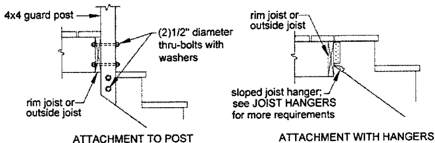
Figure 31: Stair Stringer Attachment Detail
