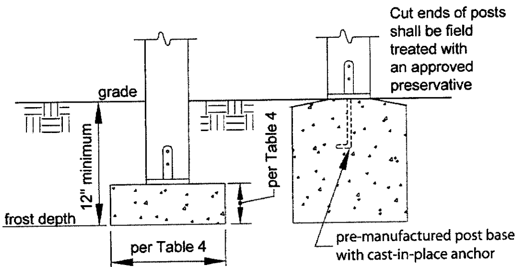
Figure 12: Typical Footing Options
