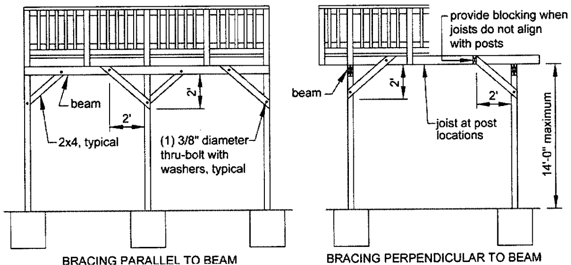
Figure 22: Diagonal Bracing Requirements
