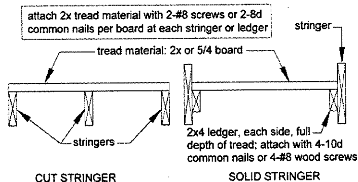
Figure 29: Tread Connection Requirements
