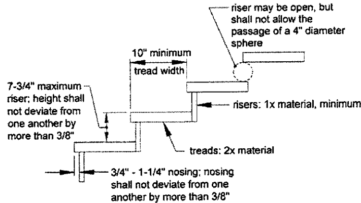
Figure 28: Stair Stringer Requirements
