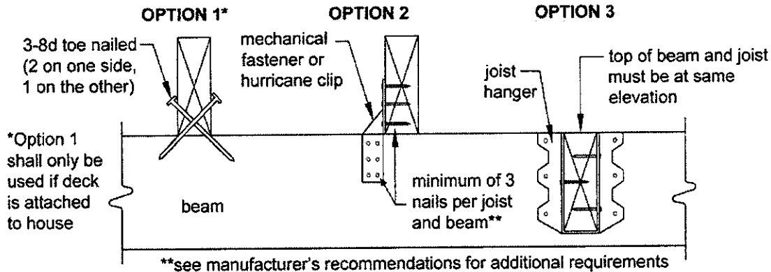
Figure 6: Joist-to-Beam Detail
