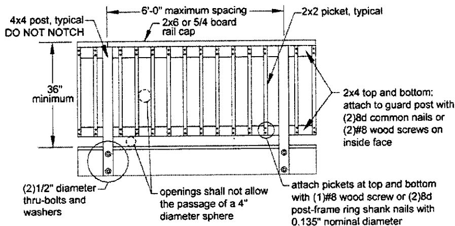
Figure 24: Typical Guard Detail
