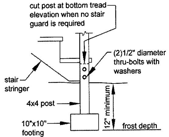
Figure 34: Stair Footing Detail
