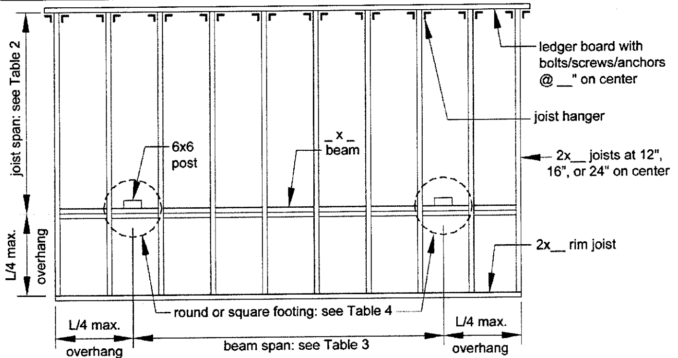
Figure 5: Typical Deck Framing Plan
