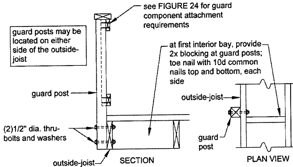
Figure 25: Guard Post to Outside Joist Detail
